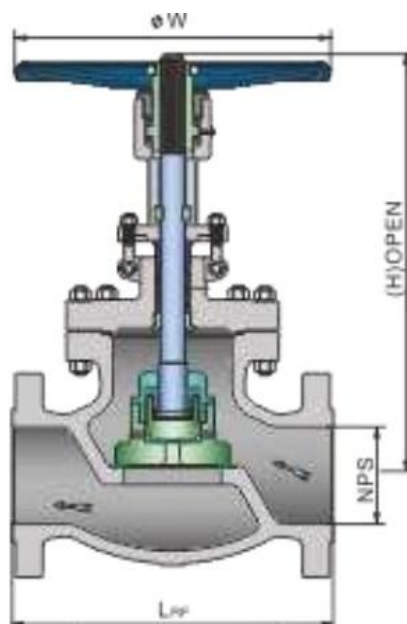
Double Disc High inlet to low outlet 150~1500LB
