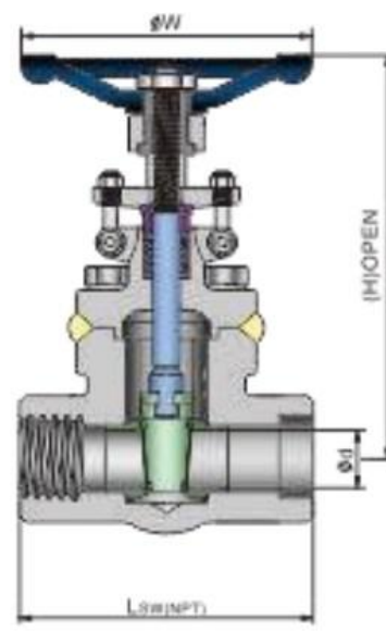
SW(NPT)WELDED BONNET 800,1500LB
