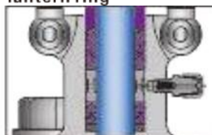
3.Grease injector & lantern ring
