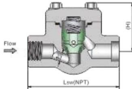
PISTON TYPE, SW(NPT) BOLTED BONNET 800, 1500LB
