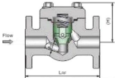
PISTON TYPE, FLANGED BOLTED BONNET 150 ~ 1500LB
