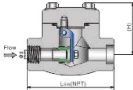
SWING TYPE, SW(NPT) BOLTED BONNET 800, 1500LB
