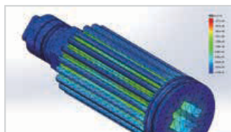
Pinion shaft analysis
