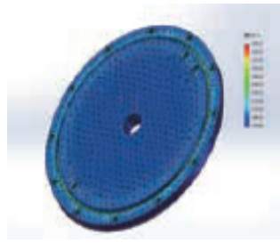
End cap stress analysis
