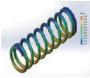
Spring fatigue stress analysis
