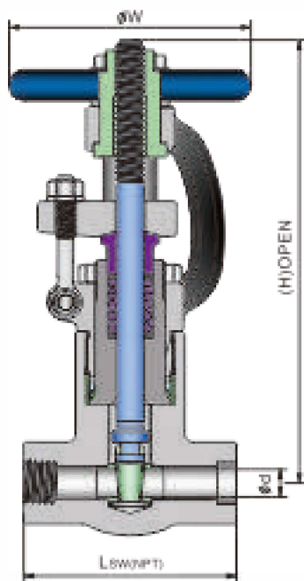
SW(NPT) PRESSURE SEAL BOMMET 1500,2500LB
